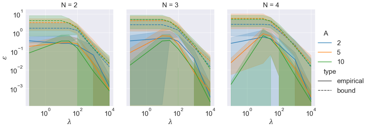
Fig. 1: Empirical vs theoretical sub-optimality of the entropy-regularized generalized Nash equilibrium (28) as a correlated equilibrium.
